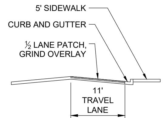
TYPICAL ROAD SECTION
