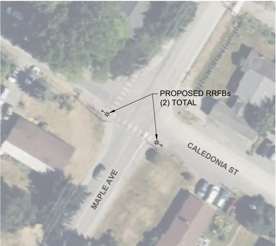
INTERSECTION OF MAPLE AVE AND CALEDONIA ST
